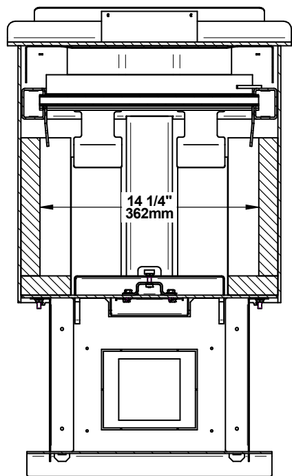
Figure 5: Front View - Firebox
