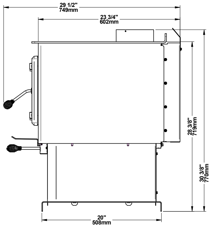
Figure 3: Side View
