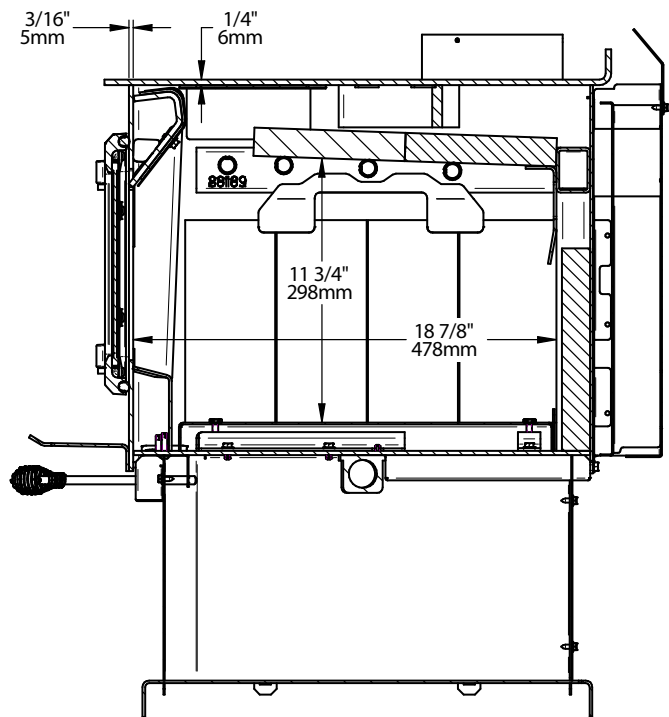
Figure 6: Side View - Firebox
