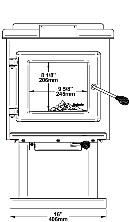
Figure 2: Front View
