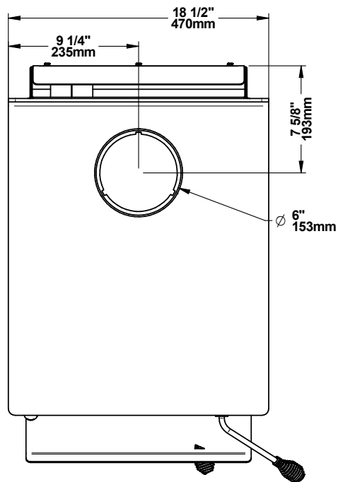
Figure 1: Top View
