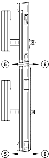
Figure 34: Eccentric hinges lateral adjustment
