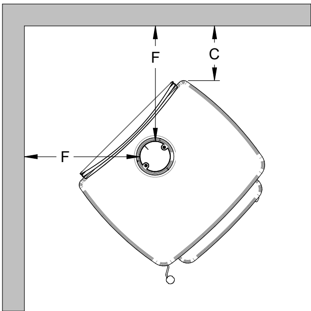
Figure 41: Clearances - Corner
