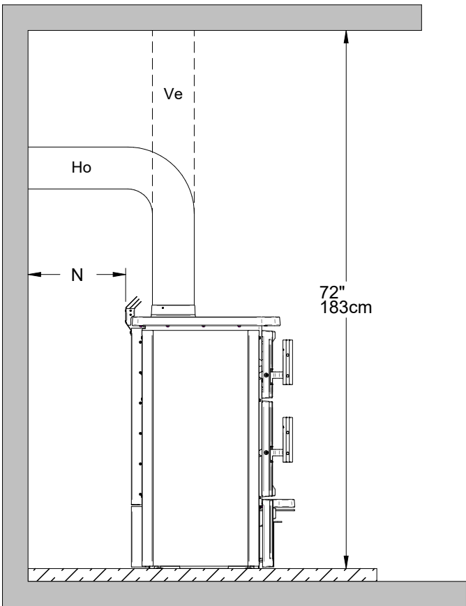
Figure 40: Clearances - Side
