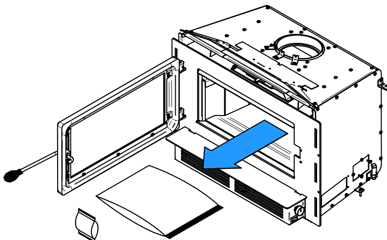
Figure 8 : Empty the combustion chamber
