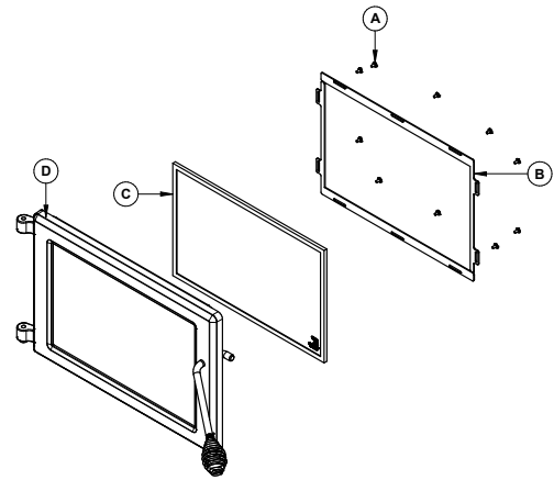
Figure 7 : Replacing the glass
