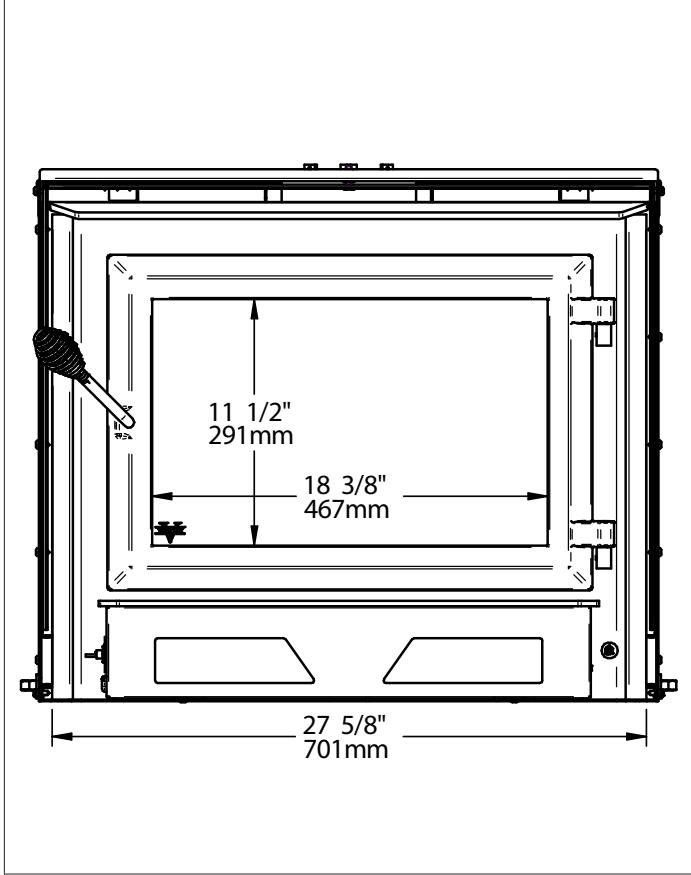
Figure 3 : Front View
