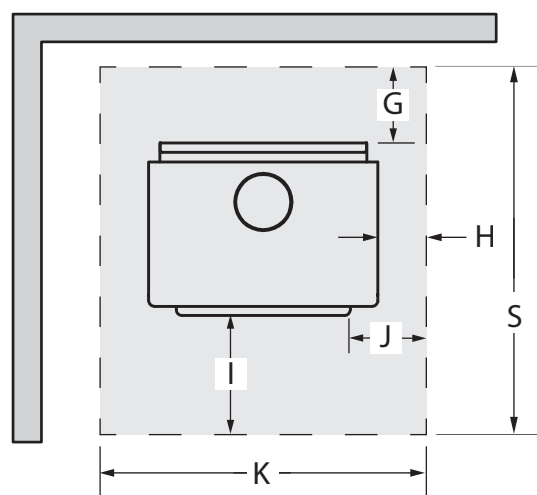
Figure 19: Protection de plancher
