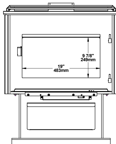
Figure 6: Door opening
