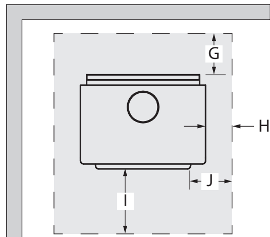
Figure 16: Protection de plancher
