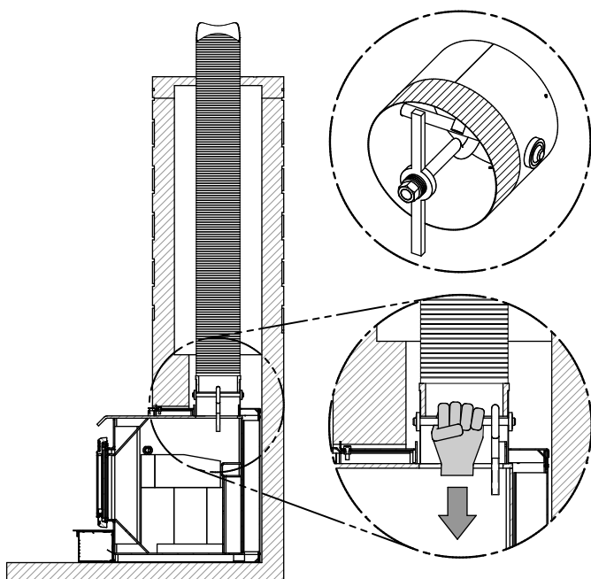
Figure 43: Liner fastening system
