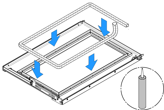
Figure 32: Door gasket
