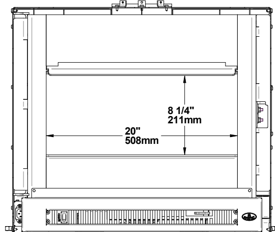
Figure 2: Door opening
