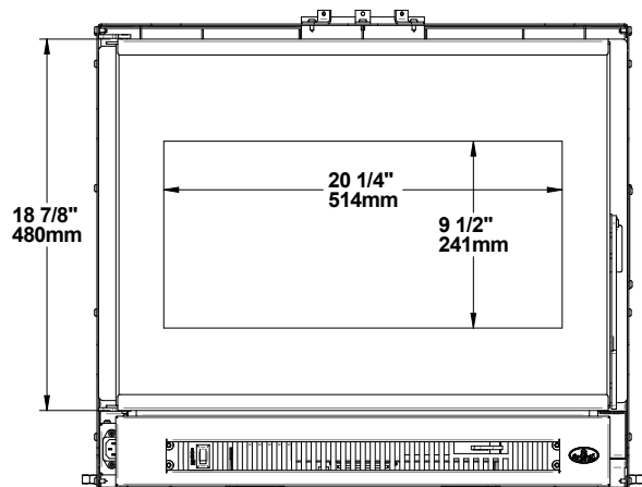
Figure 3: Front View
