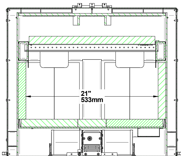
Figure 5: Front Firebox
