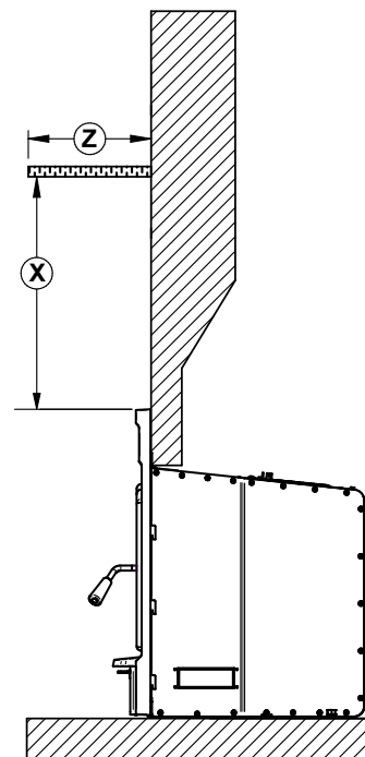
Figure 34: Shelf Clearances
