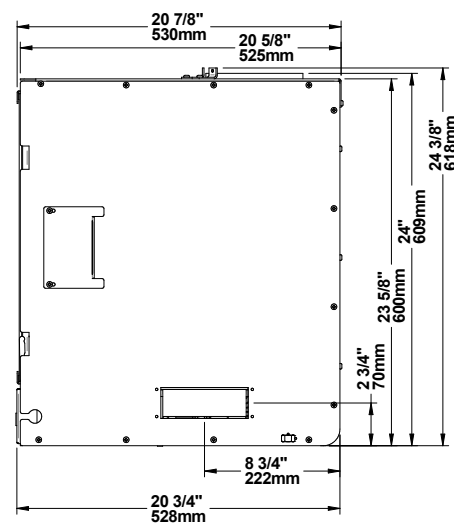
Figure 4: Side View
