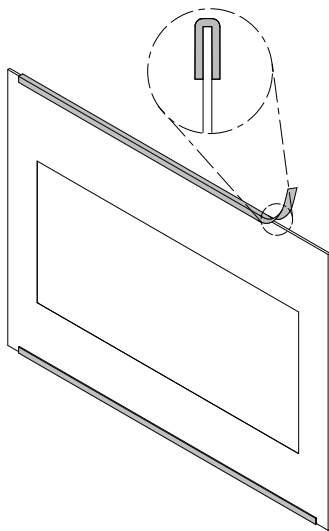
Figure 26: Glass gasket
