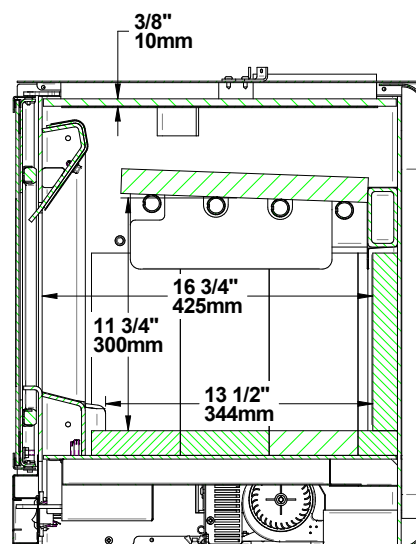
Figure 6: Side Firebox
