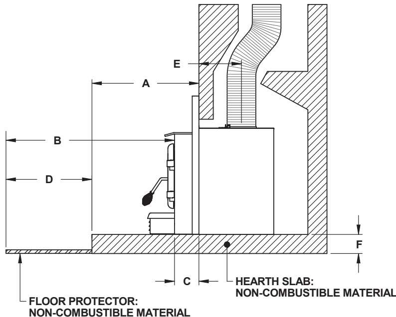
Figure 37: More than 5" raised base installation
