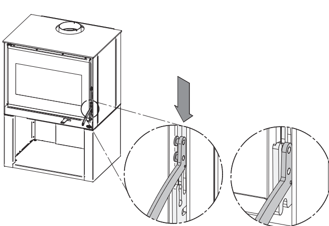
Figure 20: Opening on the right side of the insert
