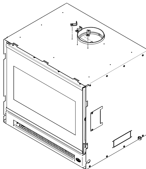
Figure 42: Securing the brackets
