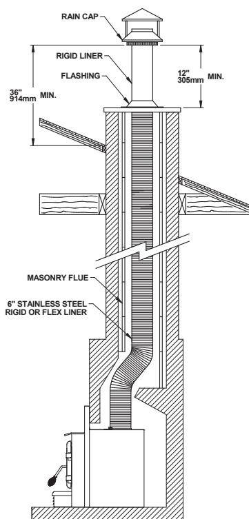
Figure 41: Liner Installation
