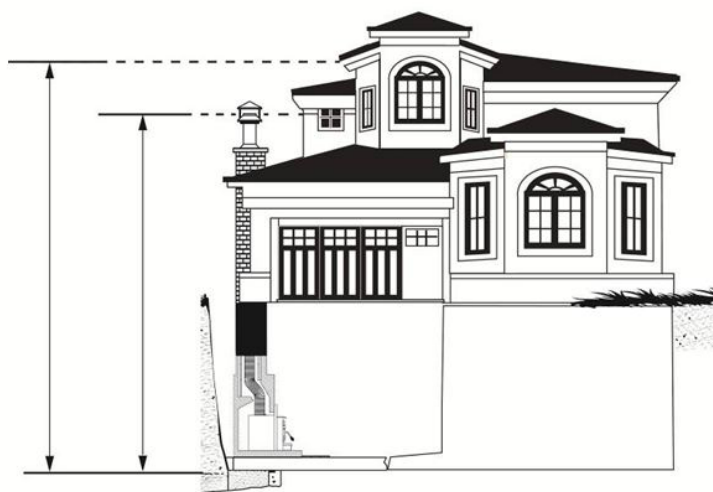
Figure 46: Chimney location in the house
